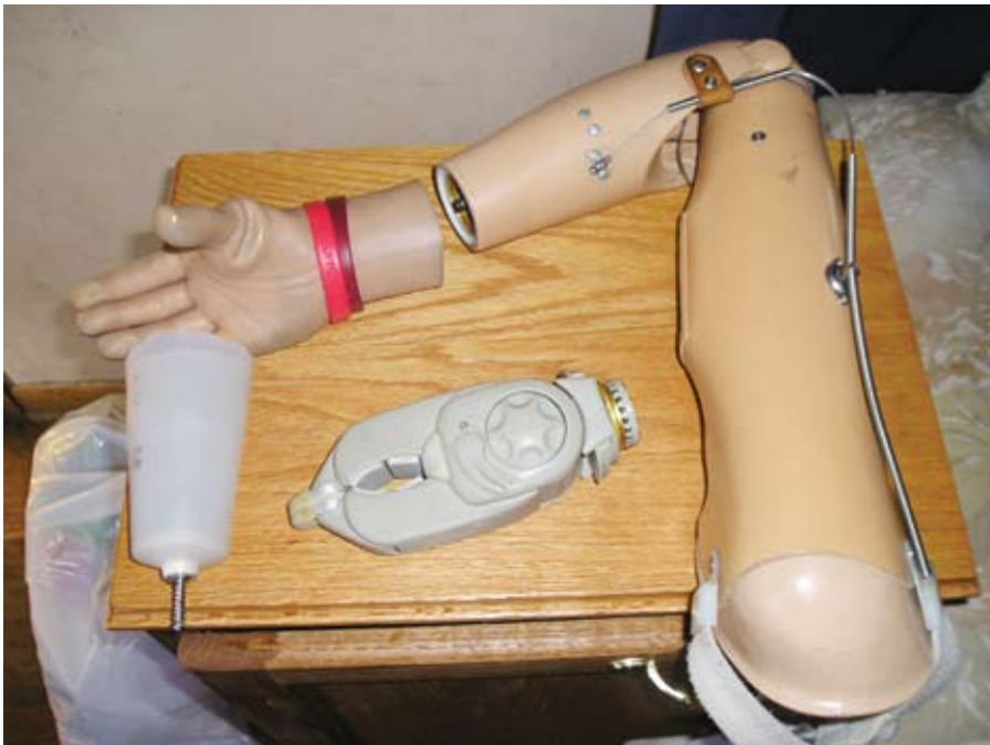
Example of hybrid above-elbow prosthesis.
